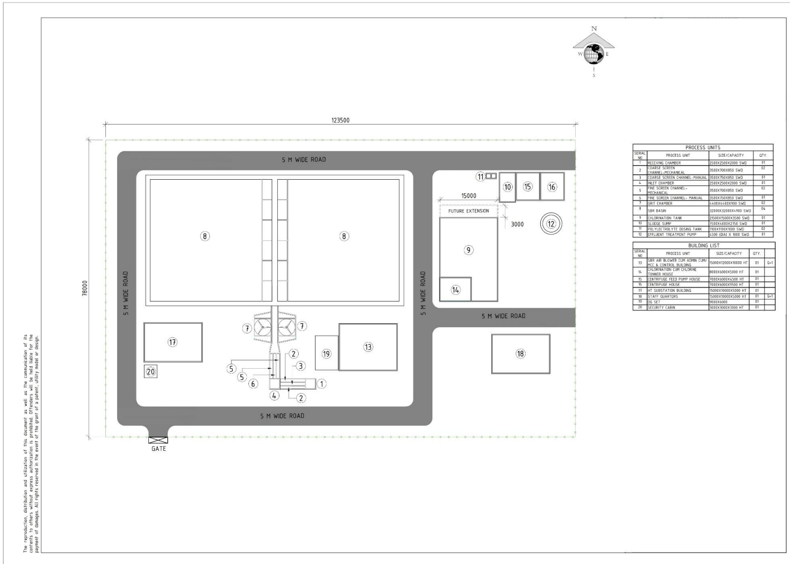
Fig. IV: Sample layout of STP
