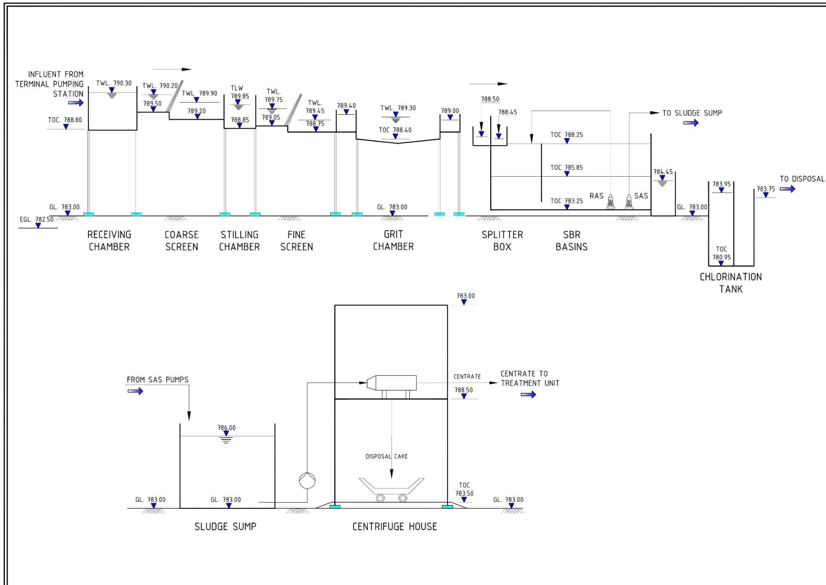
Fig. V: Sample Hydraulic Flow Diagram of STP
